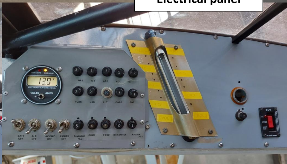
Electrical panel
